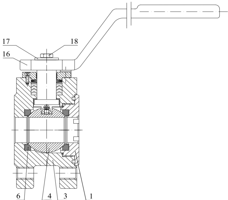
Ball valve with full bore and Flange .
